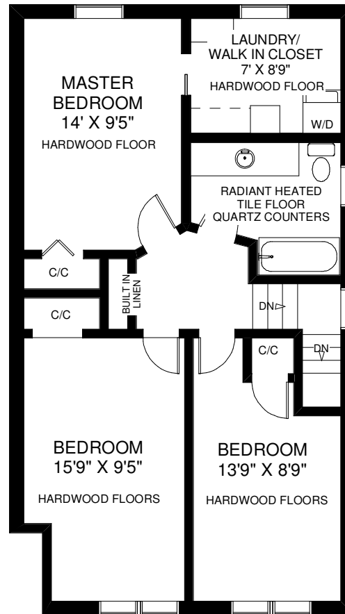
SECOND FLOOR APPROXIMATELY 750 SQ FT
