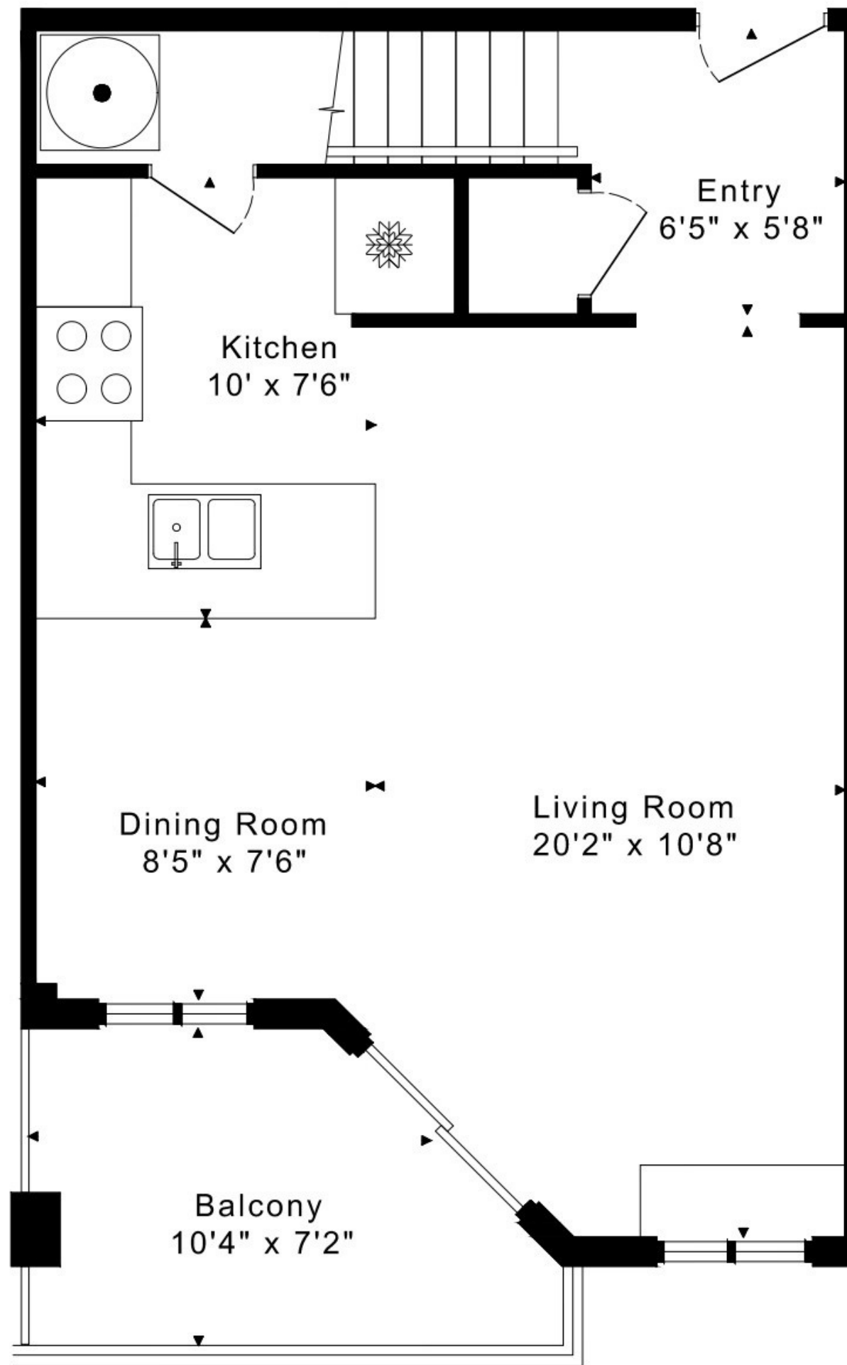
MAIN FLOOR
