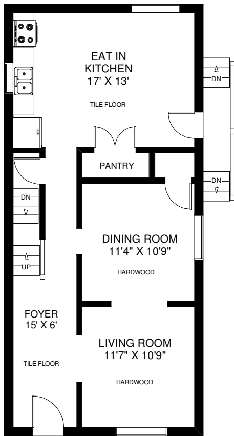
MAIN FLOOR APPROXIMATELY 780 SQ FT
