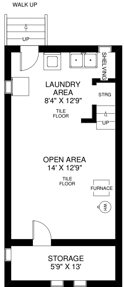
LOWER FLOOR APPROXIMATELY 450 SQ FT
