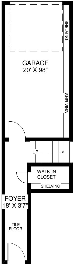
ENTRY FLOOR
