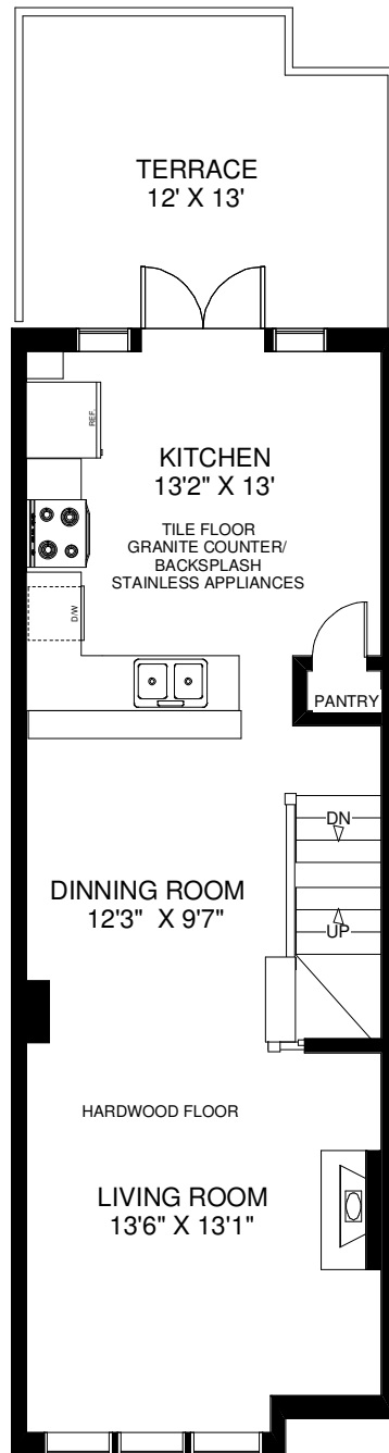
MAIN FLOOR APPROXIMATELY 560 SQ FT
