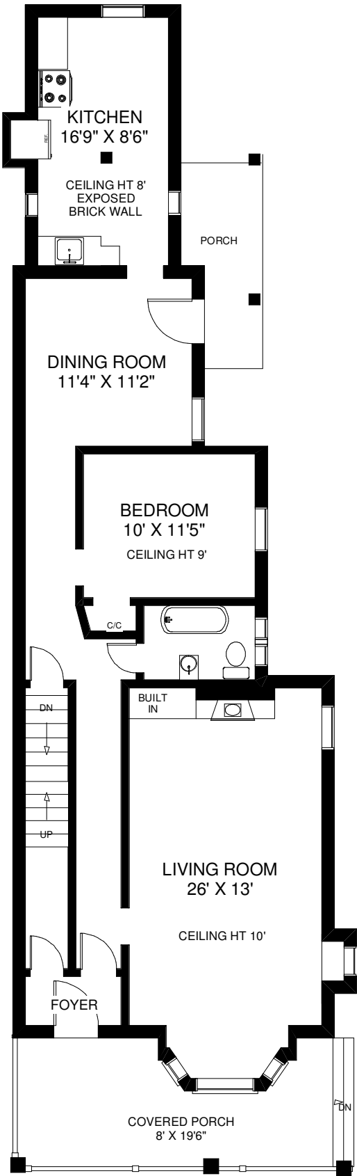
MAIN FLOOR APPROXIMATELY 1,160 SQ FT
