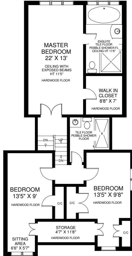
SECOND FLOOR APPROXIMATELY 1,120 SQ FT
