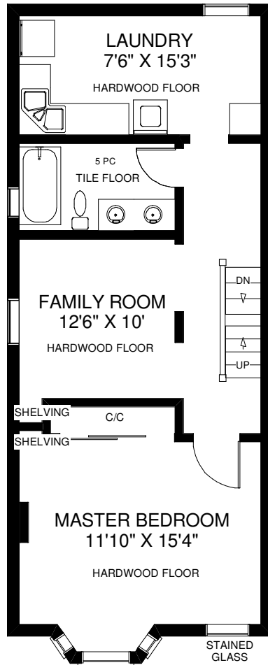
SECOND FLOOR APPROXIMATELY 700 SQ FT
