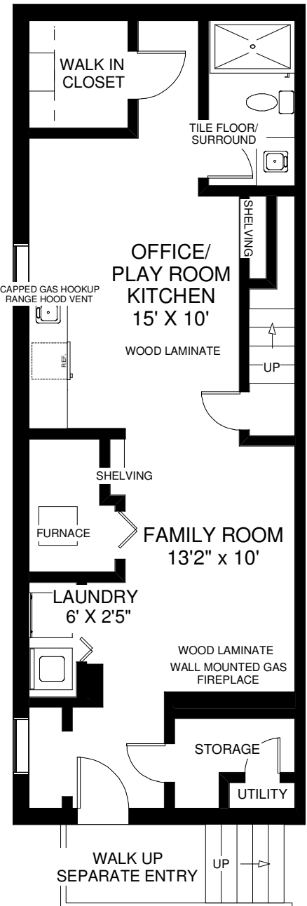
LOWER FLOOR APPROXIMATELY 650 SQ FT
