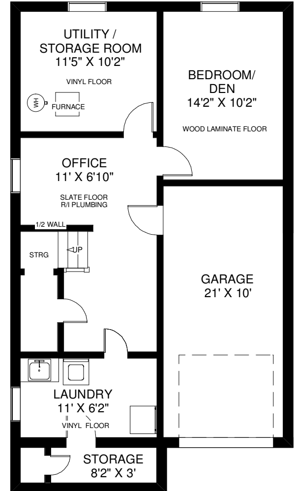
LOWER FLOOR APPROXIMATELY 720 SQ FT
