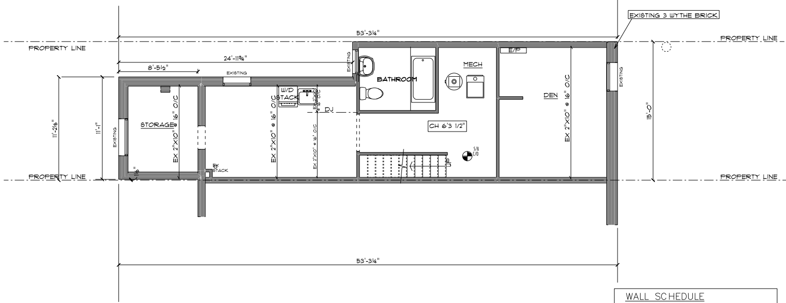
EX BASEMENT SCALE: 3/16" = 1'-0"
