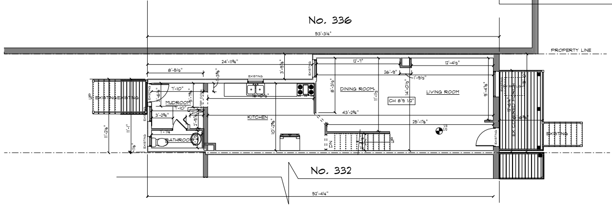
GROUND FLOOR SCALE: 0.1429" = 1'-0"
