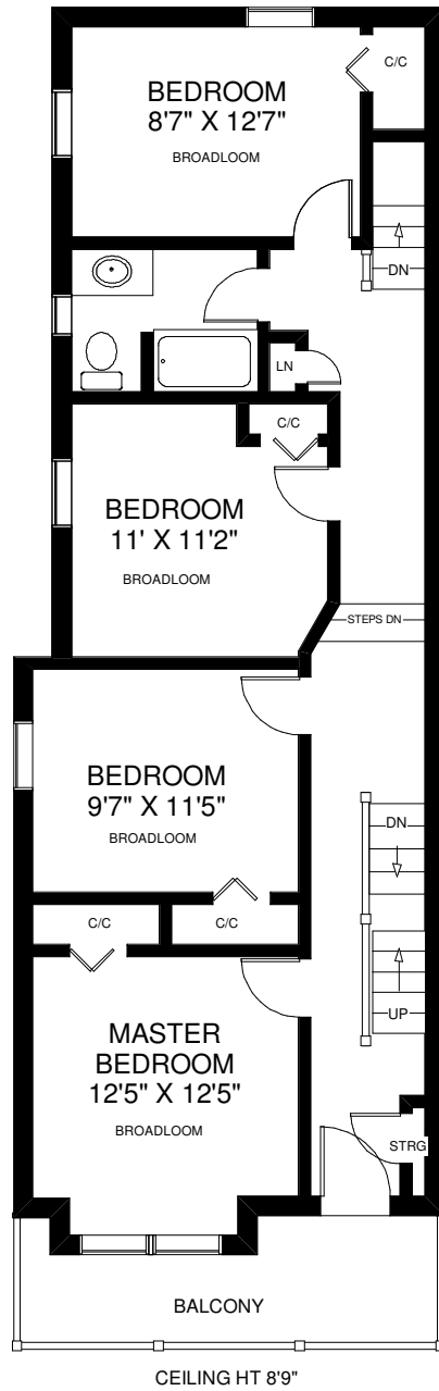
SECOND FLOOR APPROXIMATELY 935 SQ FT
