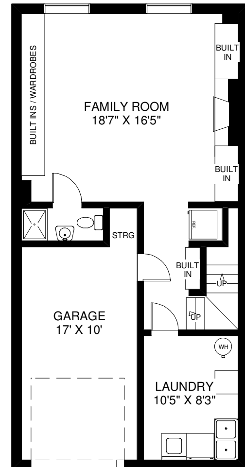
LOWER FLOOR APPROXIMATELY 600 SQ FT
