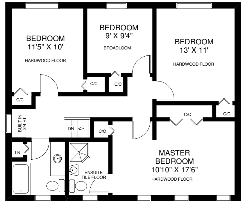
SECOND FLOOR APPROXIMATELY 900 SQ FT
