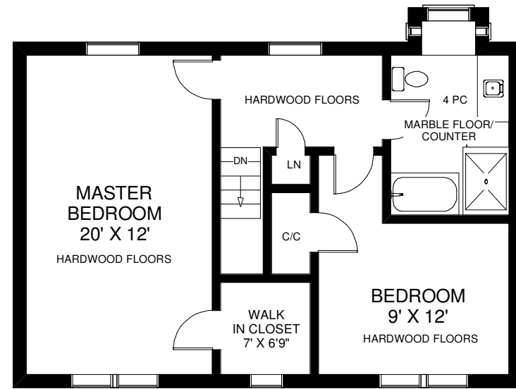
SECOND FLOOR APPROXIMATELY 720 SQ FT
