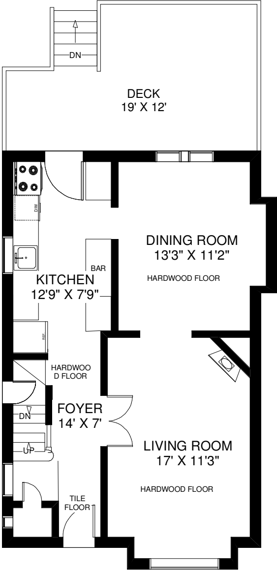
MAIN FLOOR APPROXIMATELY 650 SQ FT
