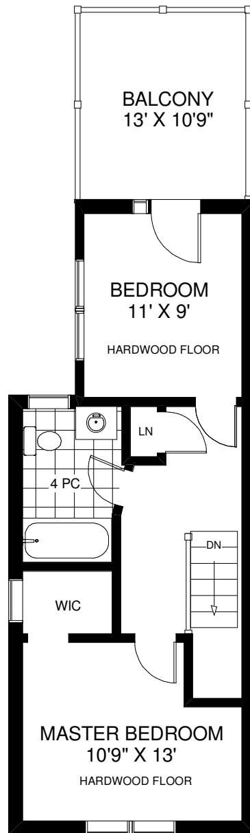
SECOND FLOOR APPROXIMATELY 530 SQ FT
